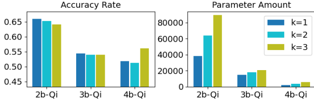
Figure 5: The accuracy of experimental results and the number of model parameters of the QiMLP at different k values under the CIFAR-10 dataset.
