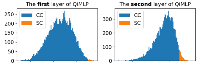
Figure 6: The proportion of classical correlations (CC) and mined strong correlations (SC) in each neuron layer of QiMLP under the MNIST dataset.
